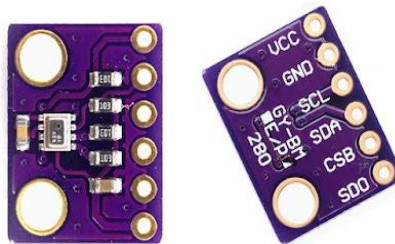
Gambar 4. Sensor BMP280
