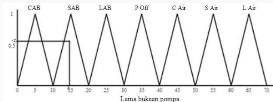
Gambar 6. Mumbership function pada output logika fuzzy, dimana LAB = Lama Nutrisi AB, SAB = Sedang Nutrisi AB, CAB = Cepat Nutrisi AB, P Off = Pompa mati, C Air = Cepat Air, S Air = Sedang Air, L Air = Lama Air.
