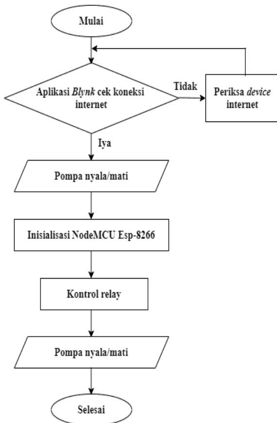
Gambar 7. Flowchart System Hidroponik NFT
